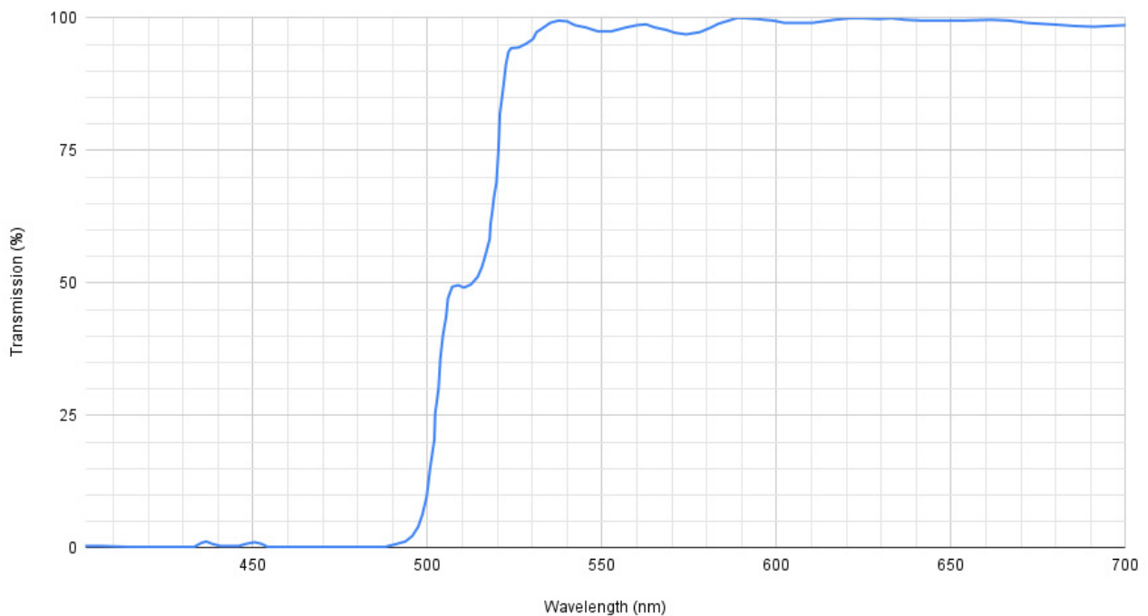
Dichroic Filter "LP500"
