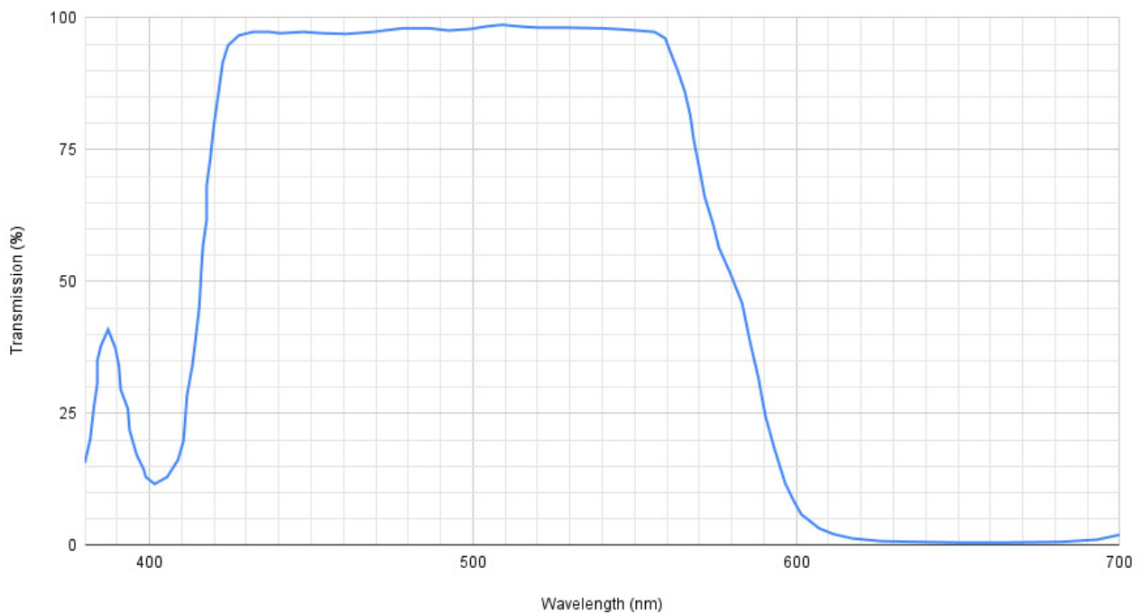
Dichroic Filter "refl. red pass green/blue"
